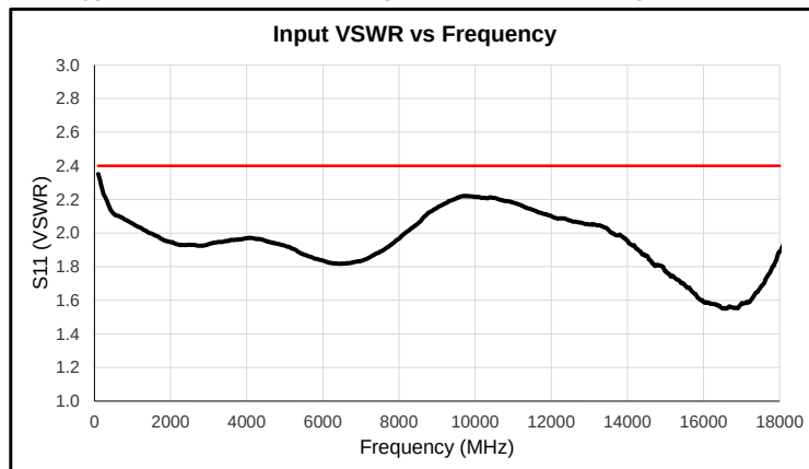
Typical Performance @ 23°C (Reference S/N 2162302)
